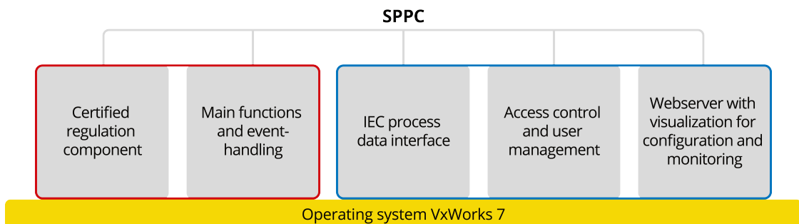
▼ Software structure of Smart Power Plant Controller on the M200 Controller
