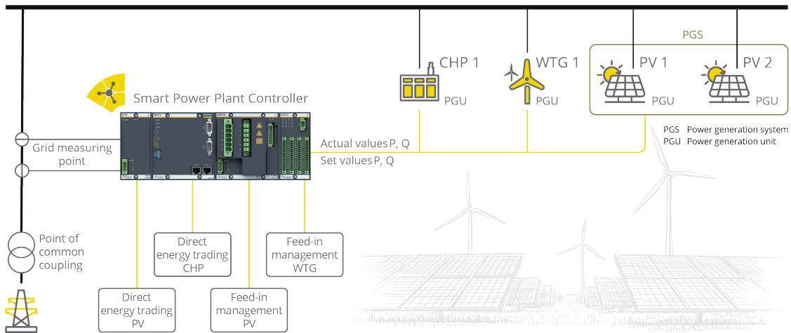
▼ Connection example of a Smart Power Plant Controller system (schematic)
