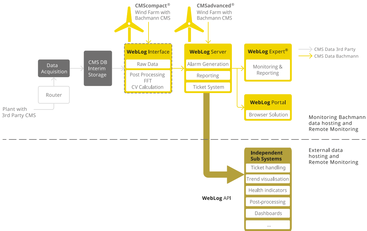
Fig. 4: Processing of measurement data provided via API on an external WebLog Server
