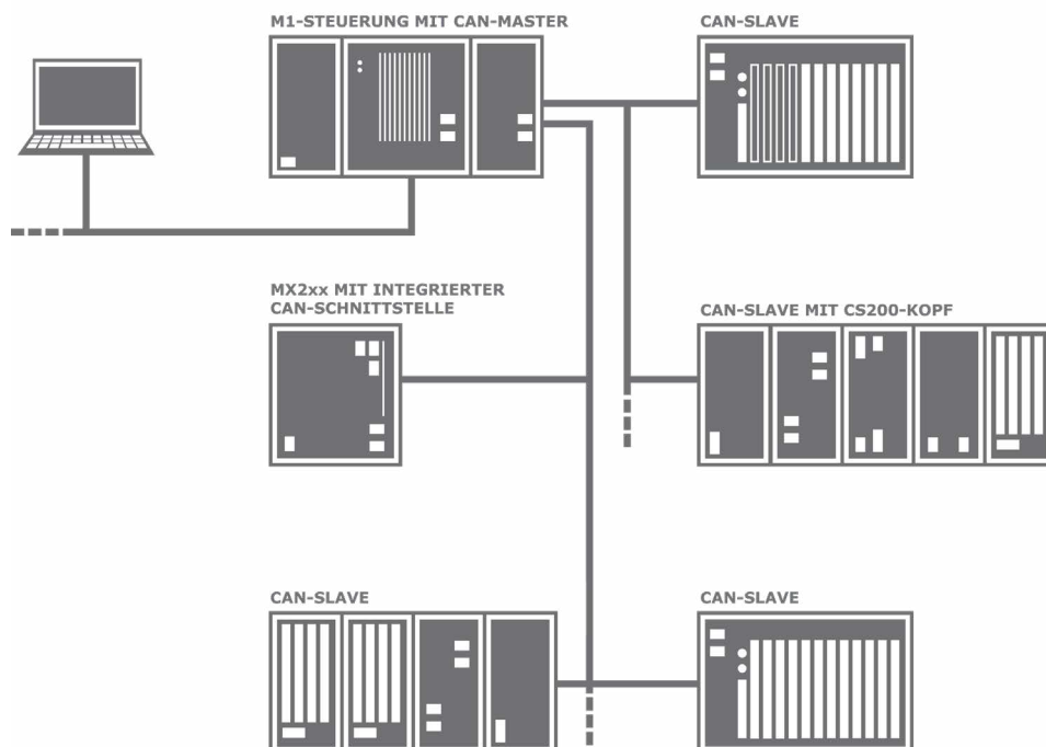
▼ Possible topology: CANopen
